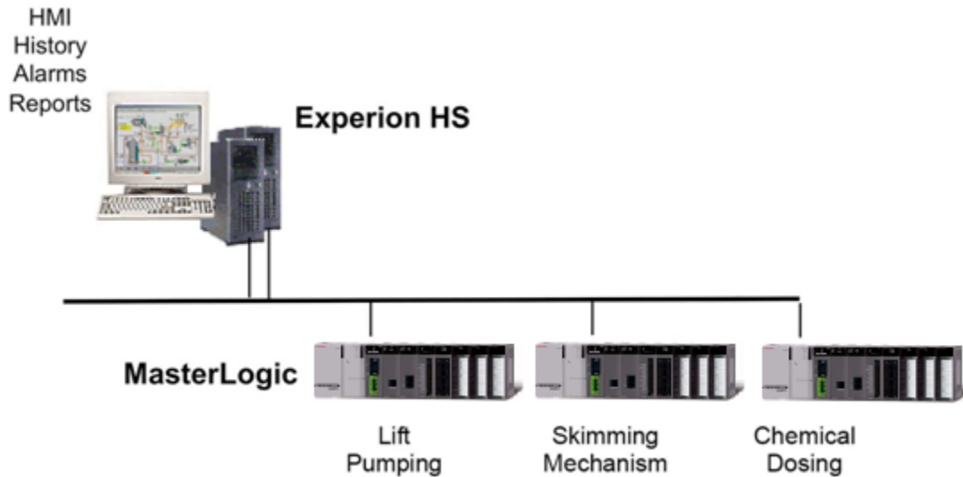
Figure 5. In balance-of-plant applications, a MasterLogic PLC can be installed on each equipment unit and networked with an Experion HS supervisory computer.
