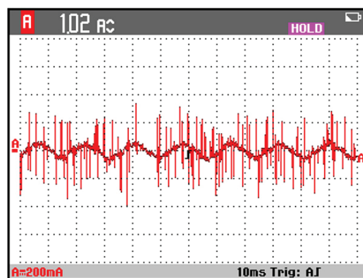
Sigma current
